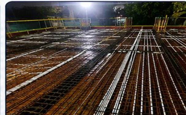
CONDUIT LAYOUT WORK IN PROGRESS
